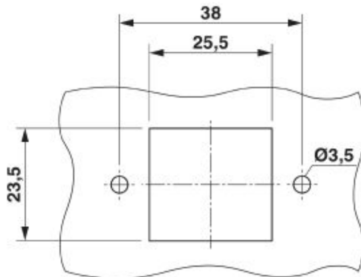
Dimensional drawing
