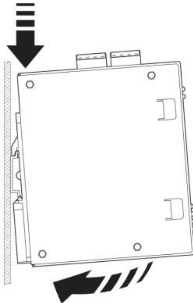
Schematic diagram
