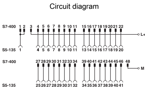
Connection scheme: FLKM S135/S400/SO120
