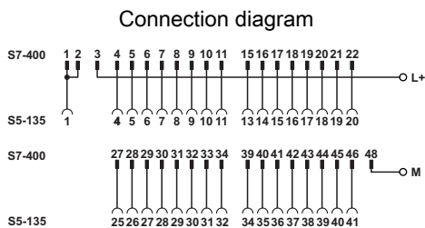
Connection scheme: FLKM S135/S400/SO120
