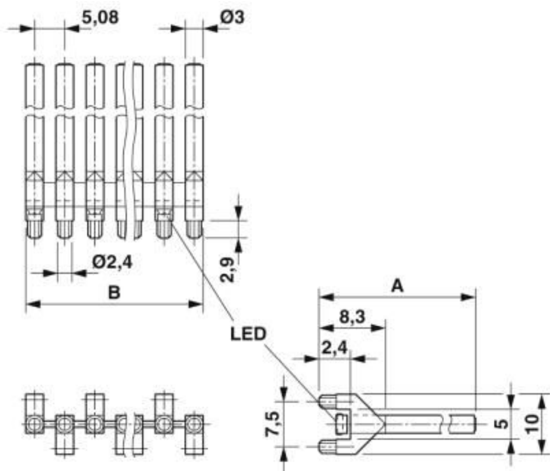
Dimensional drawing
