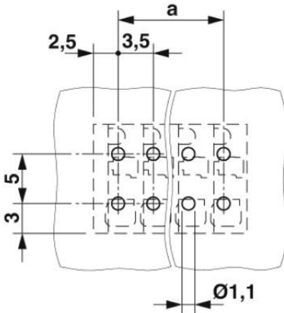
Drilling diagram
