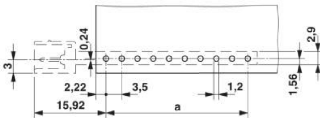
Drilling diagram
