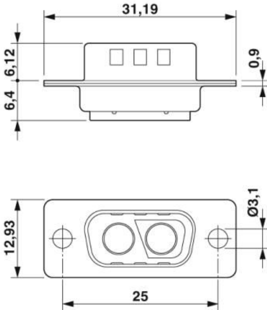
Dimensional drawing
