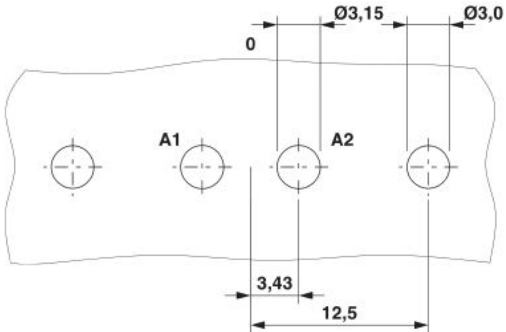
Drilling diagram
