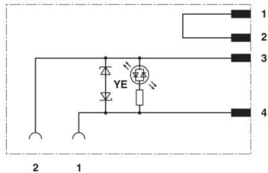
Circuit diagram
