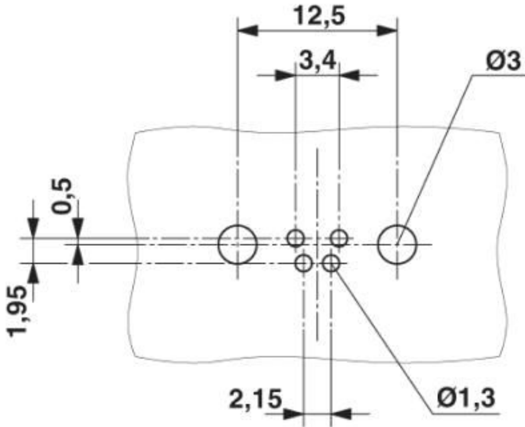
Drilling diagram
