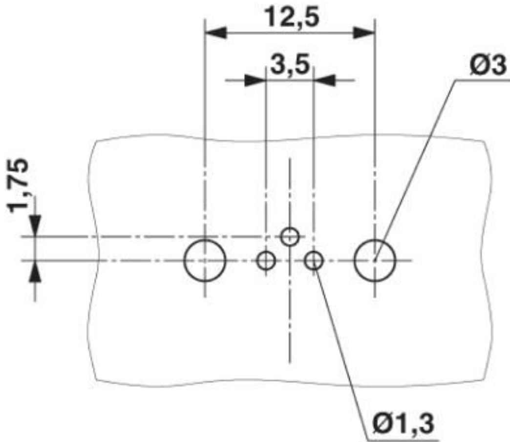
Drilling diagram
