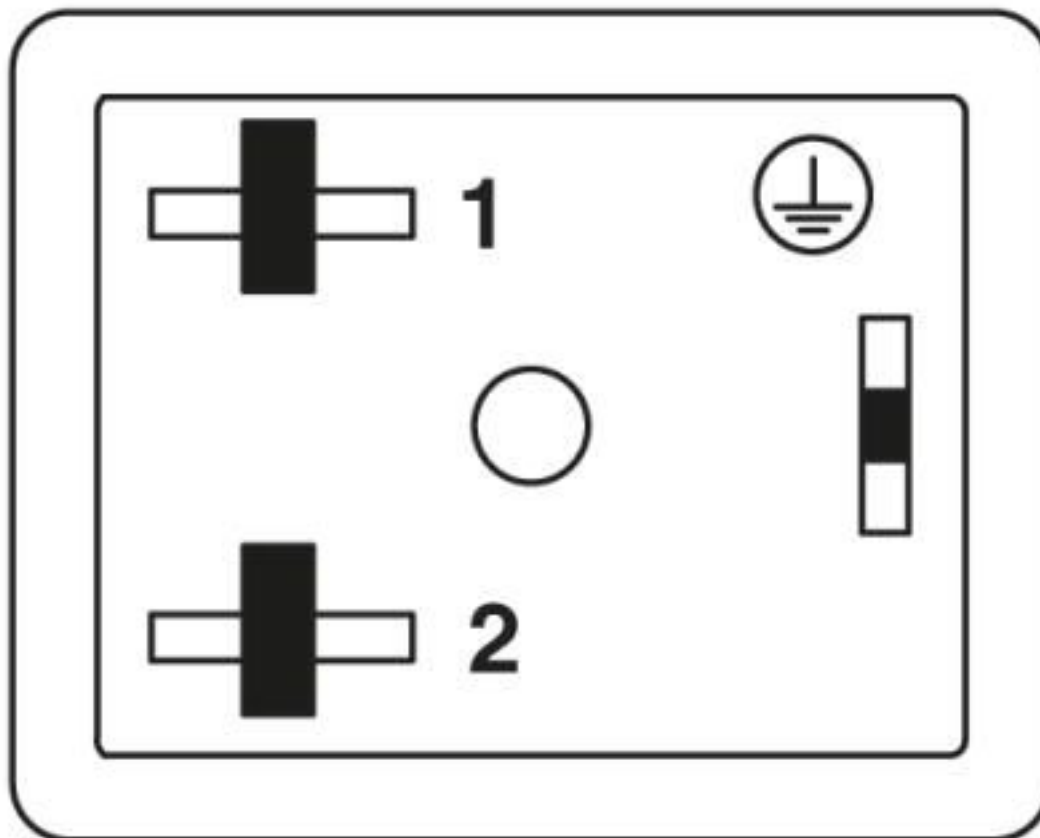
Valve connector pin assignment, type BI
