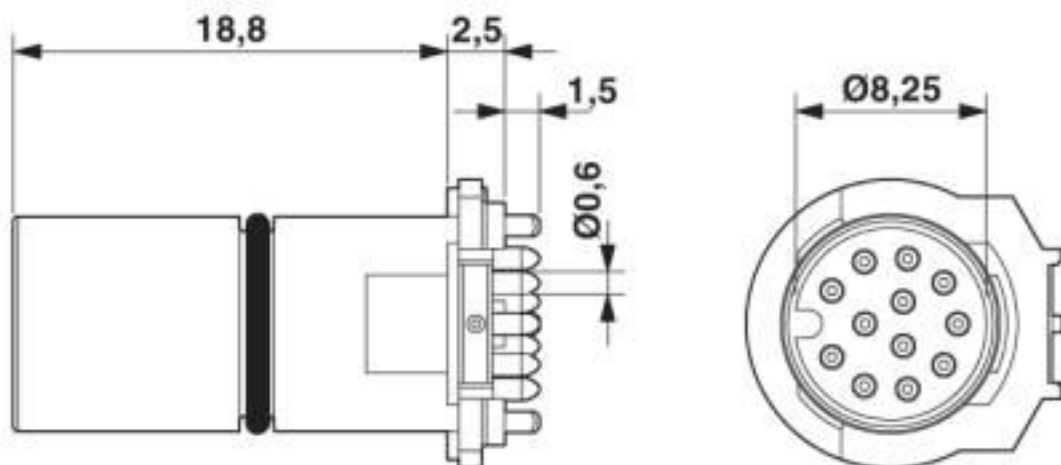
M12 flush-type connector
