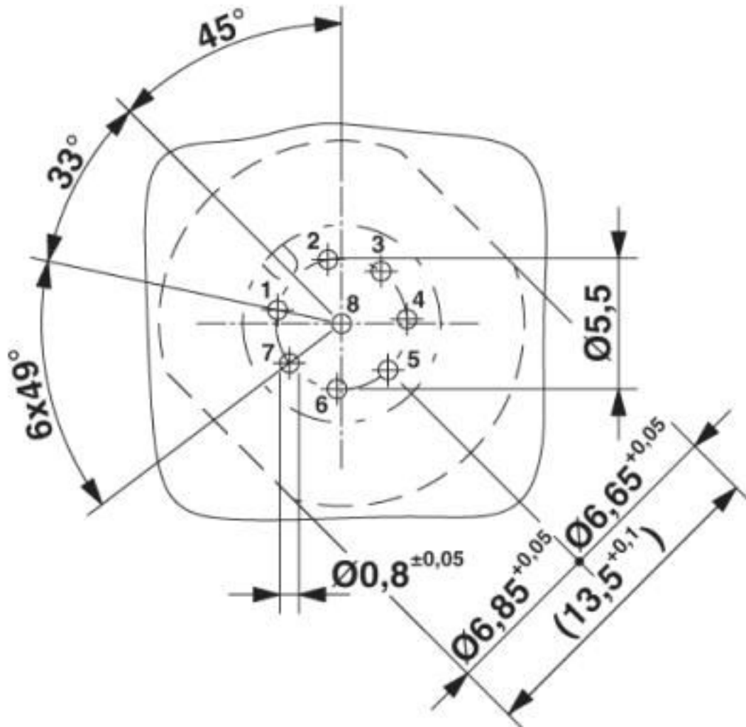
Drilling diagram
