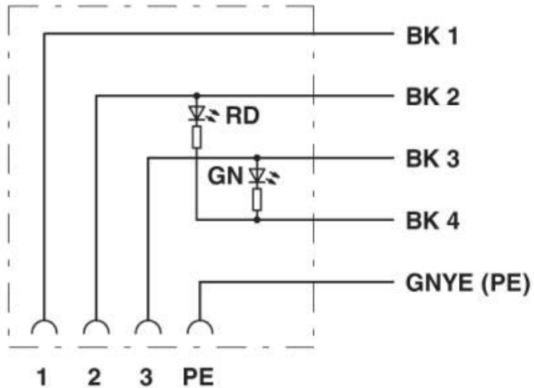
Circuit diagram
