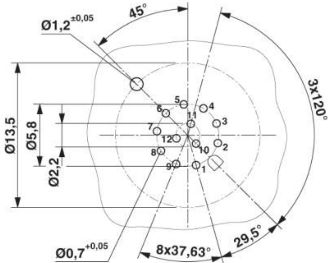
Drilling diagram
