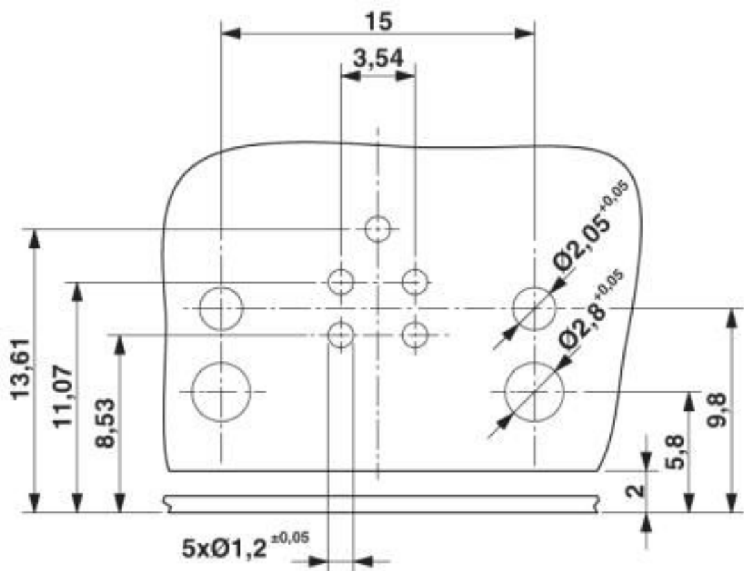
Drilling diagram
