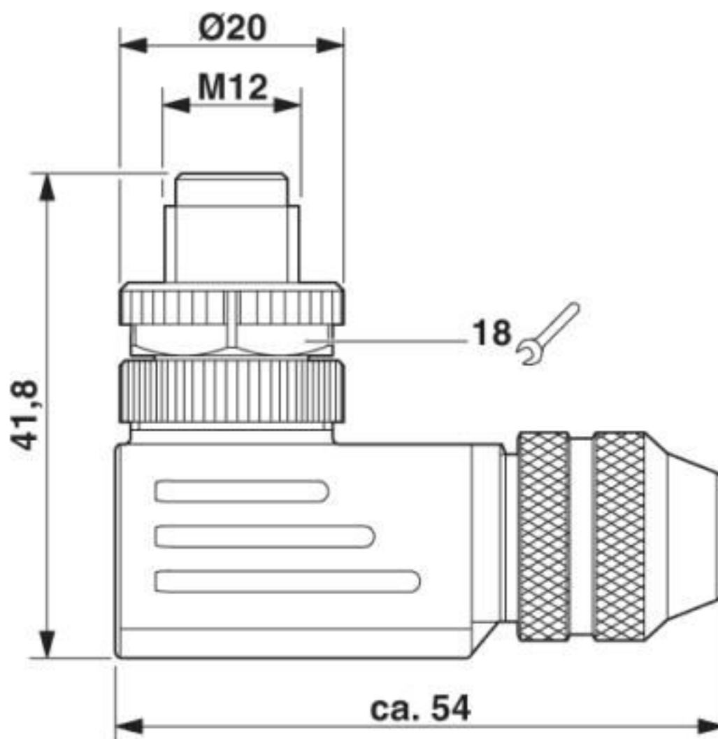
Dimensional drawing
