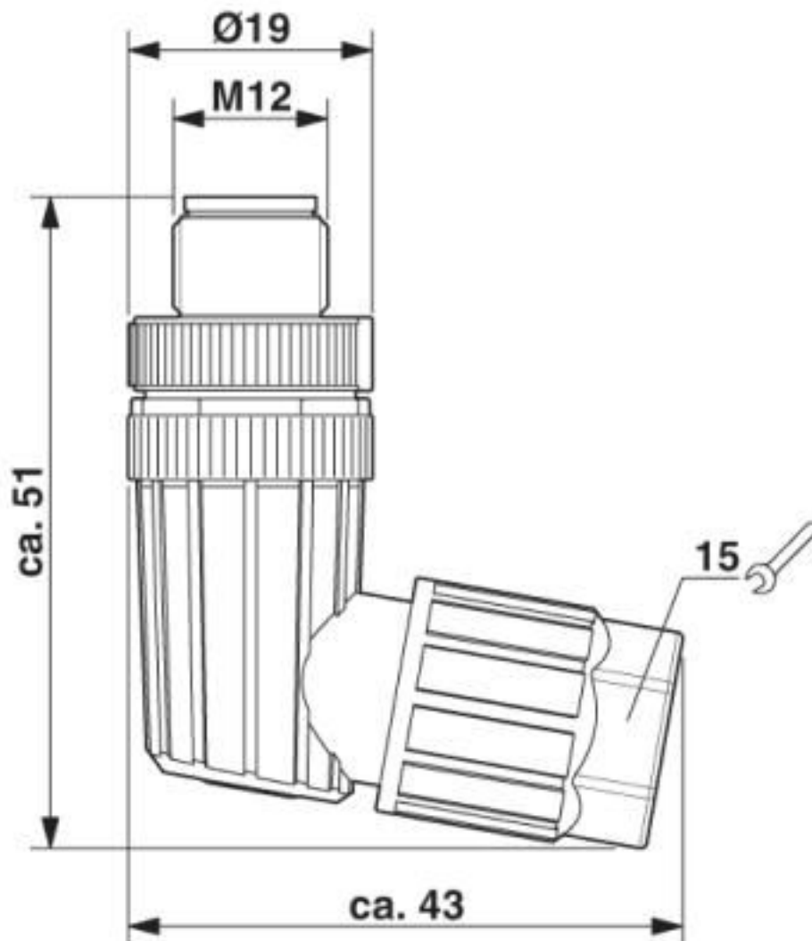
Dimensional drawing
