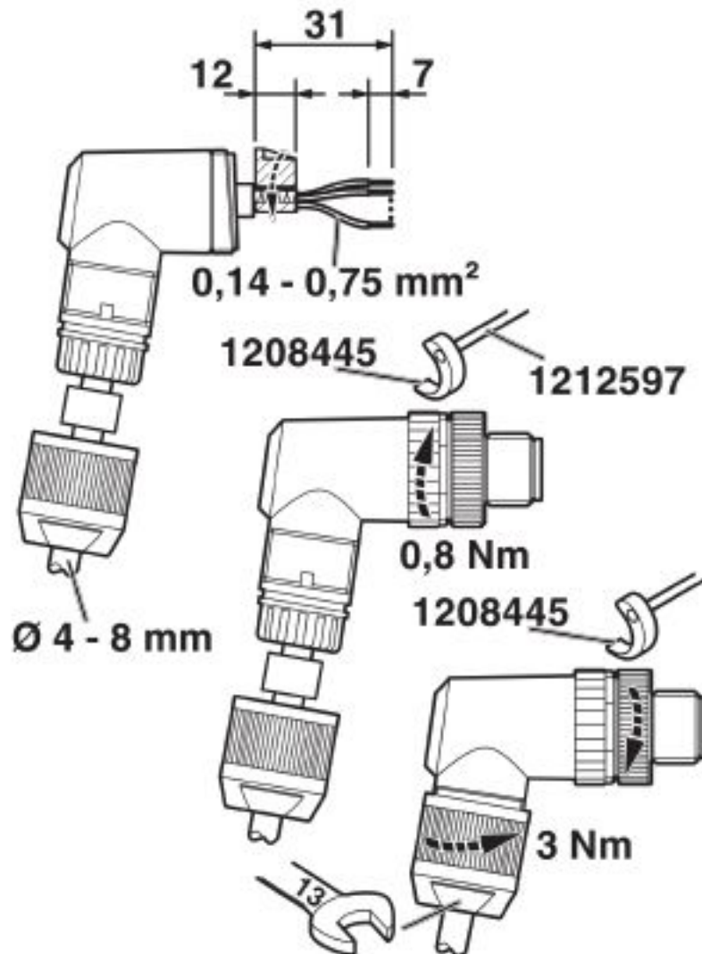
Functional drawing
