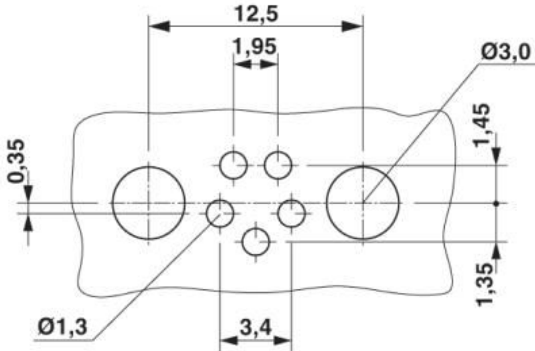
Drilling diagram
