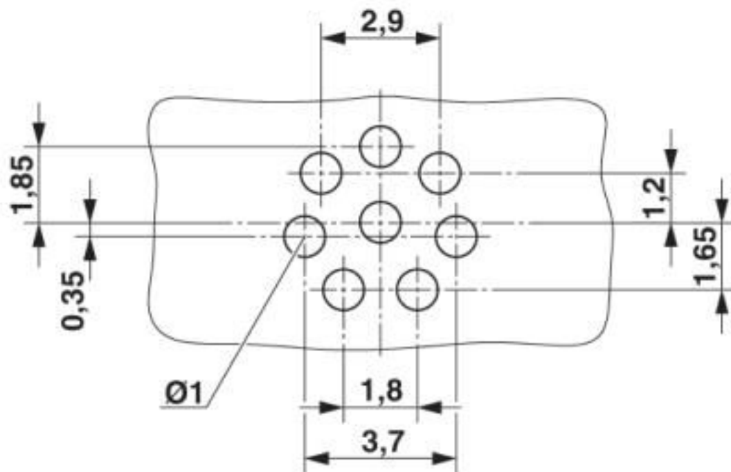
Drilling diagram
