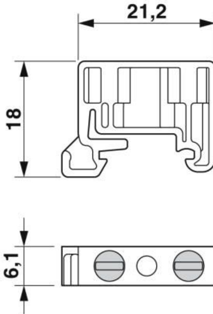
Dimensional drawing
