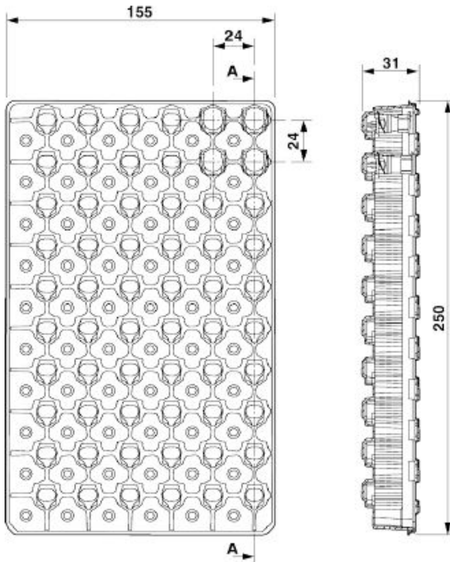
Dimensional drawing
