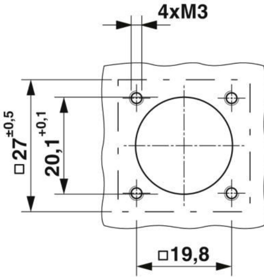
Dimensional drawing
