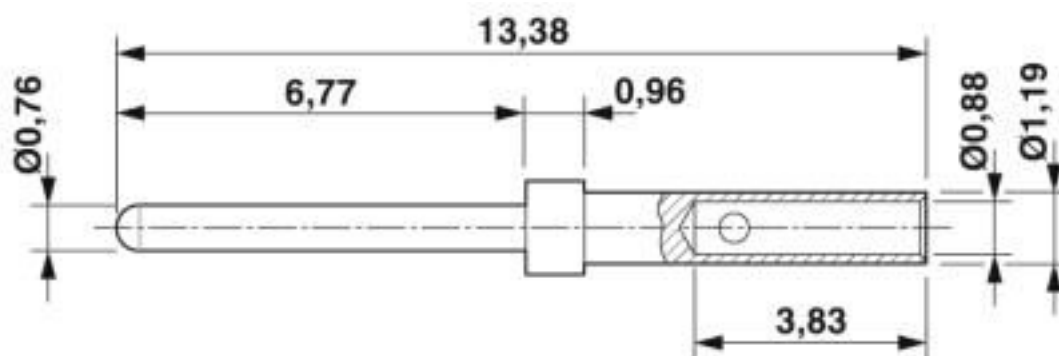
D-SUB crimp contact pin
