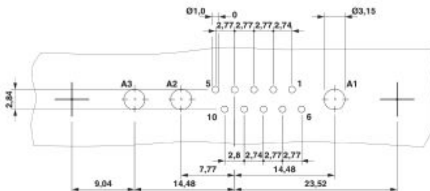
Drilling diagram
