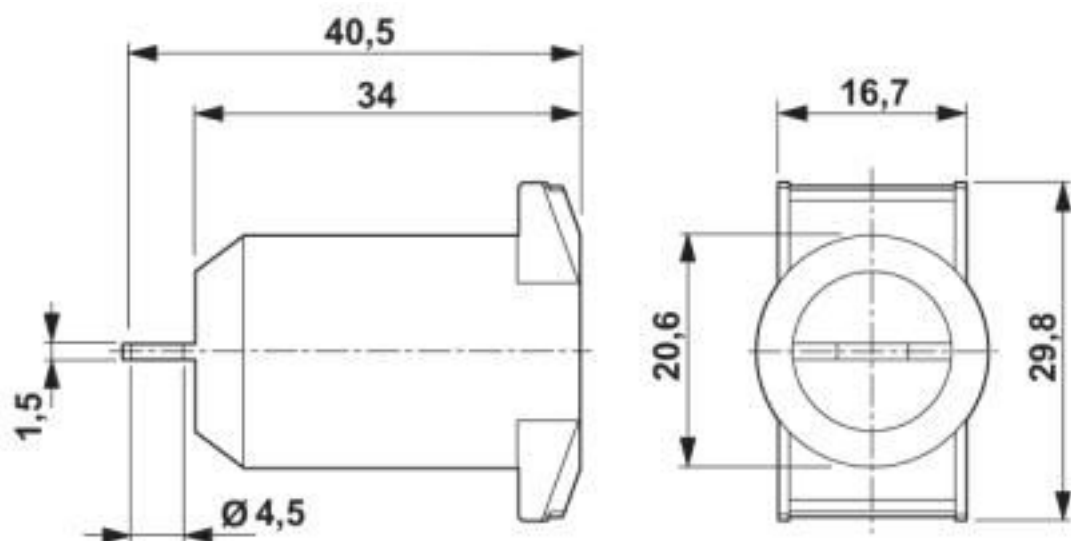
Dimensional drawing
