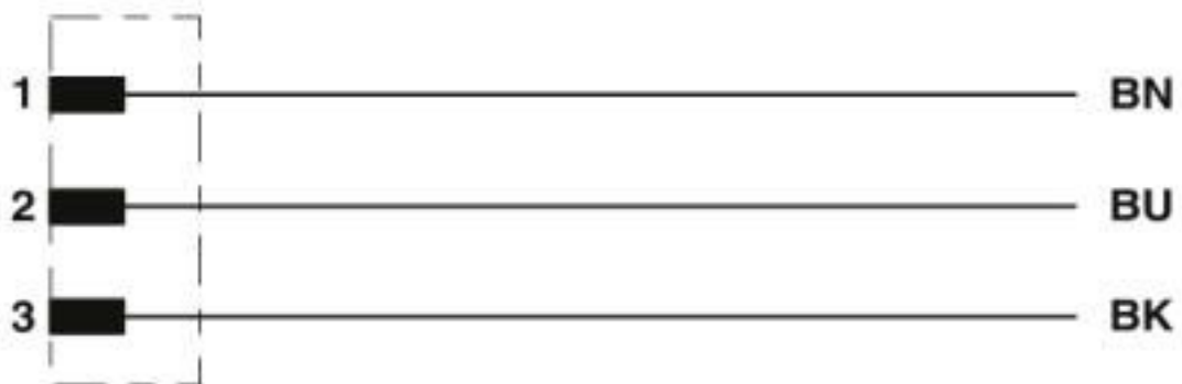
Contact assignment of the DEUTSCH DT04-3P
