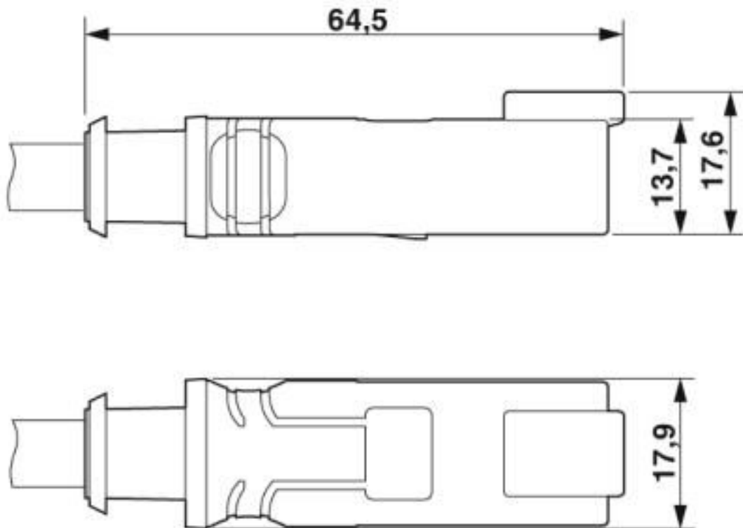
DEUTSCH DT04-2P, top view and side view
