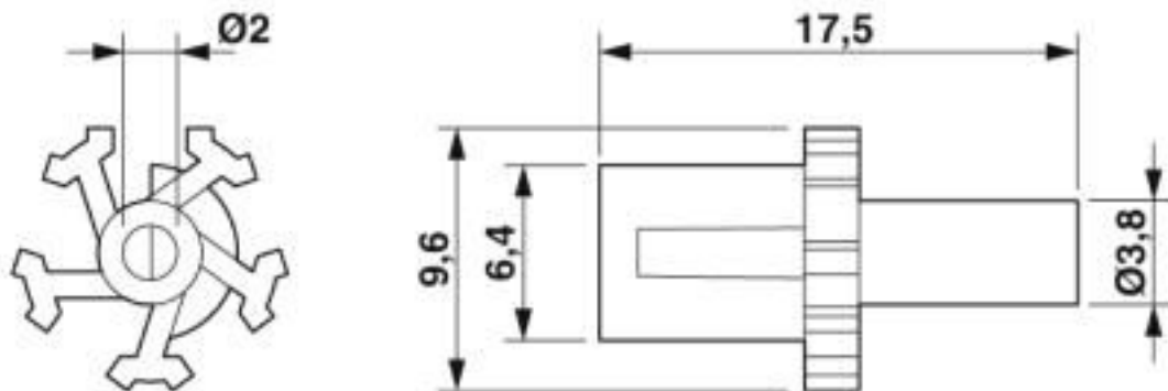
Schematic diagram
