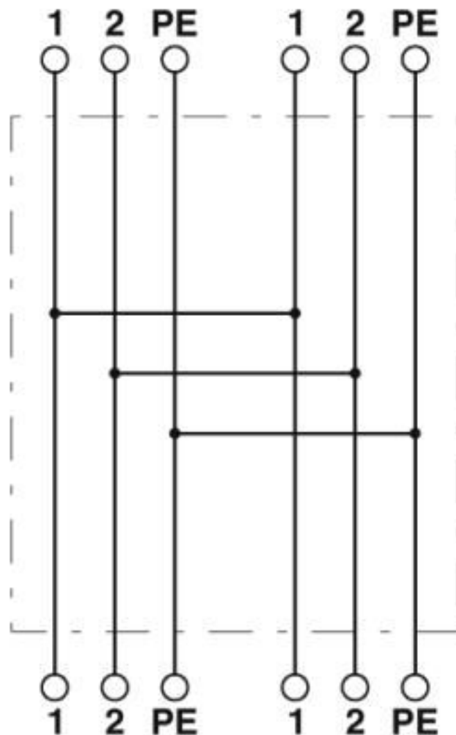
Circuit diagram
