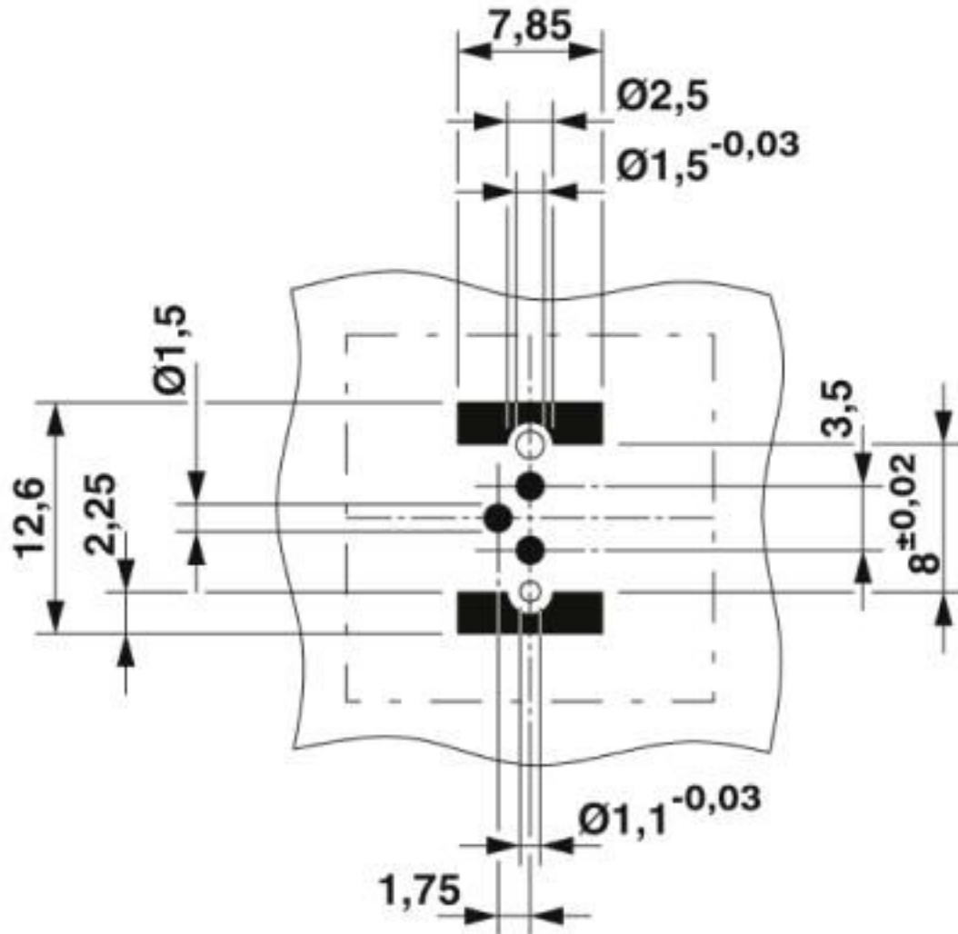
Drilling diagram
