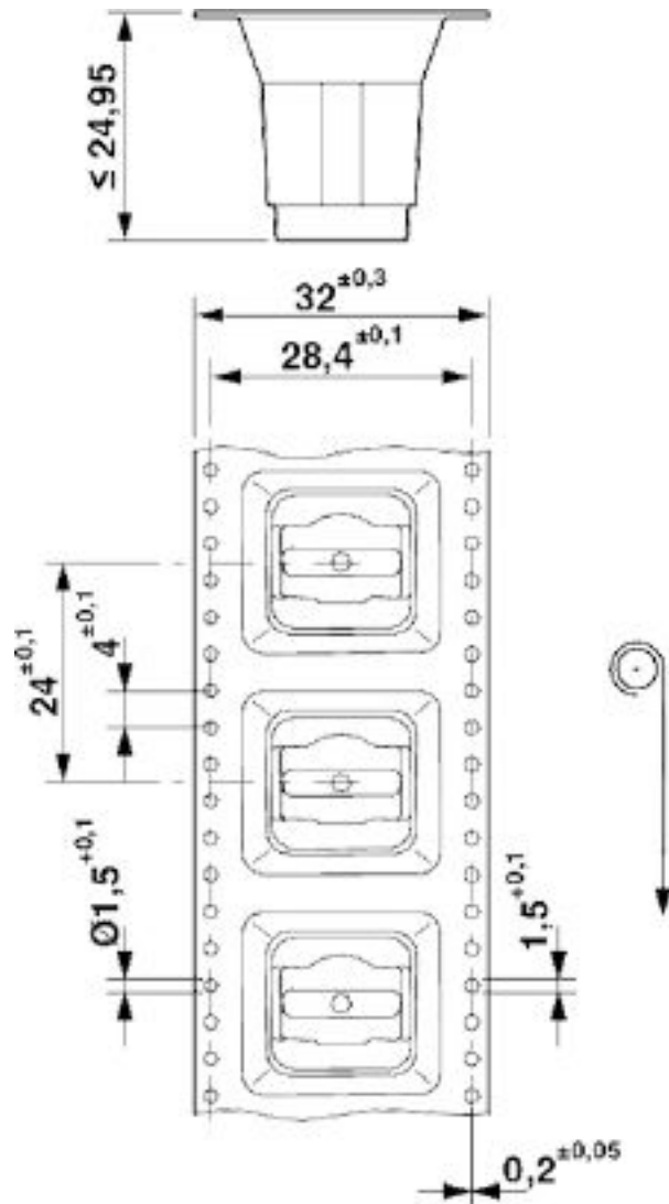
Dimensional drawing
