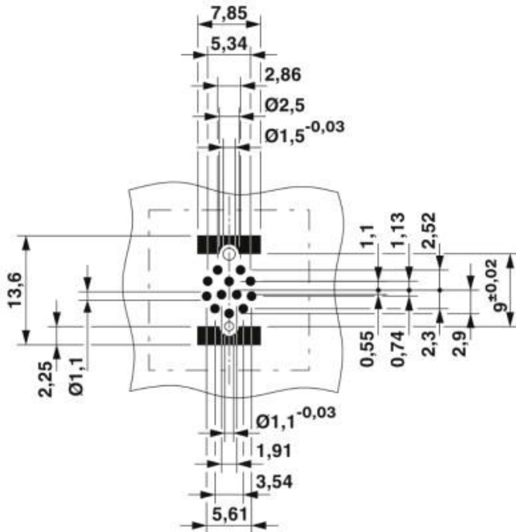
Drilling diagram
