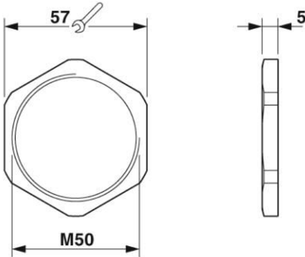
Dimensional drawing
