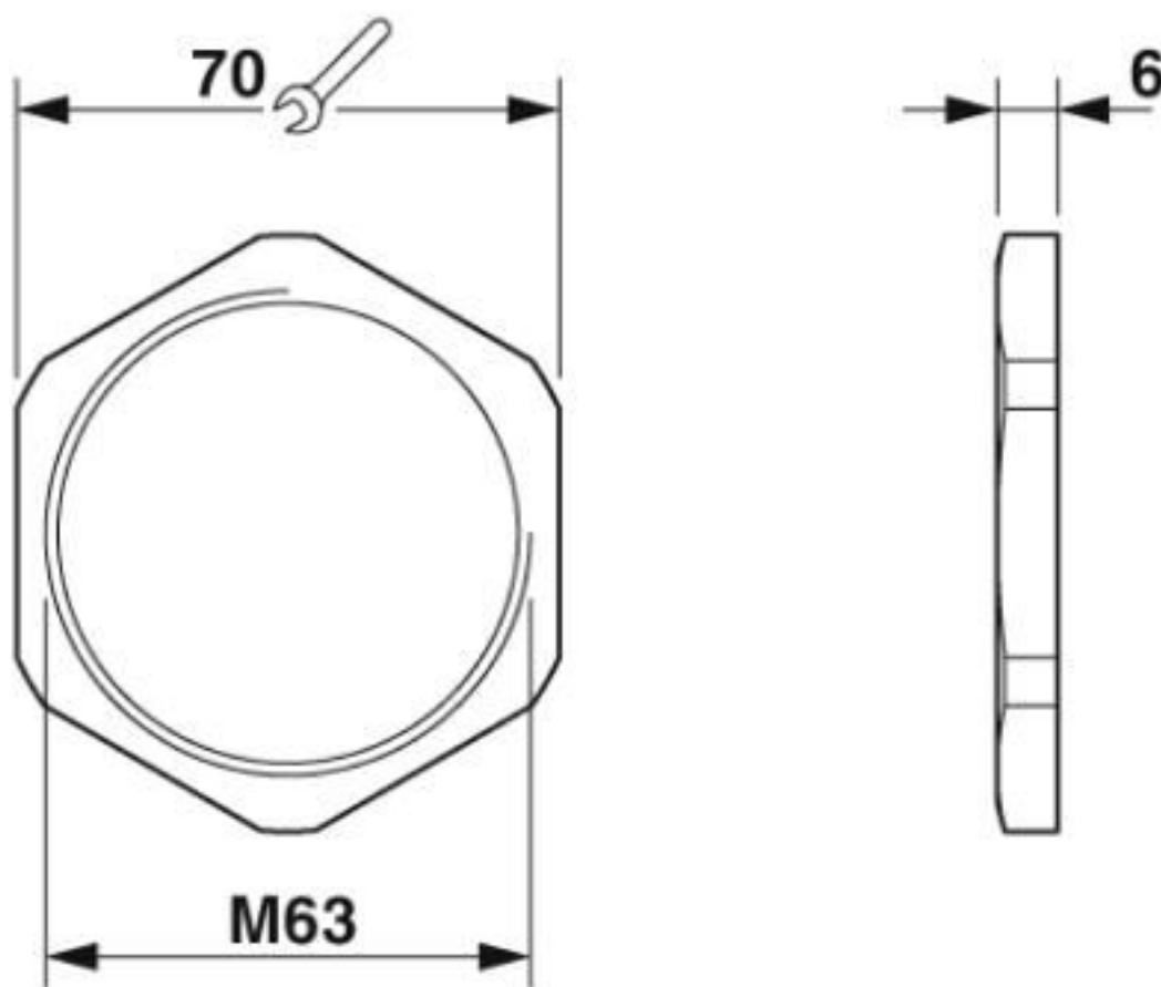
Dimensional drawing
