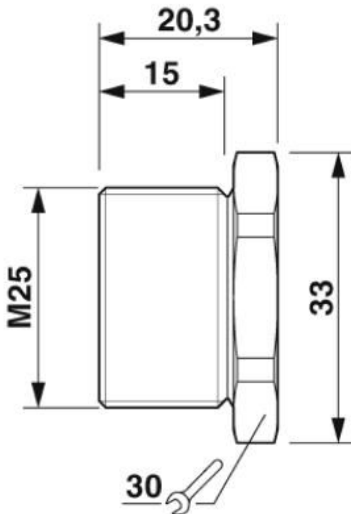
Dimensional drawing
