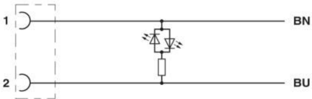
Contact assignment of the DEUTSCH DT06-2S
