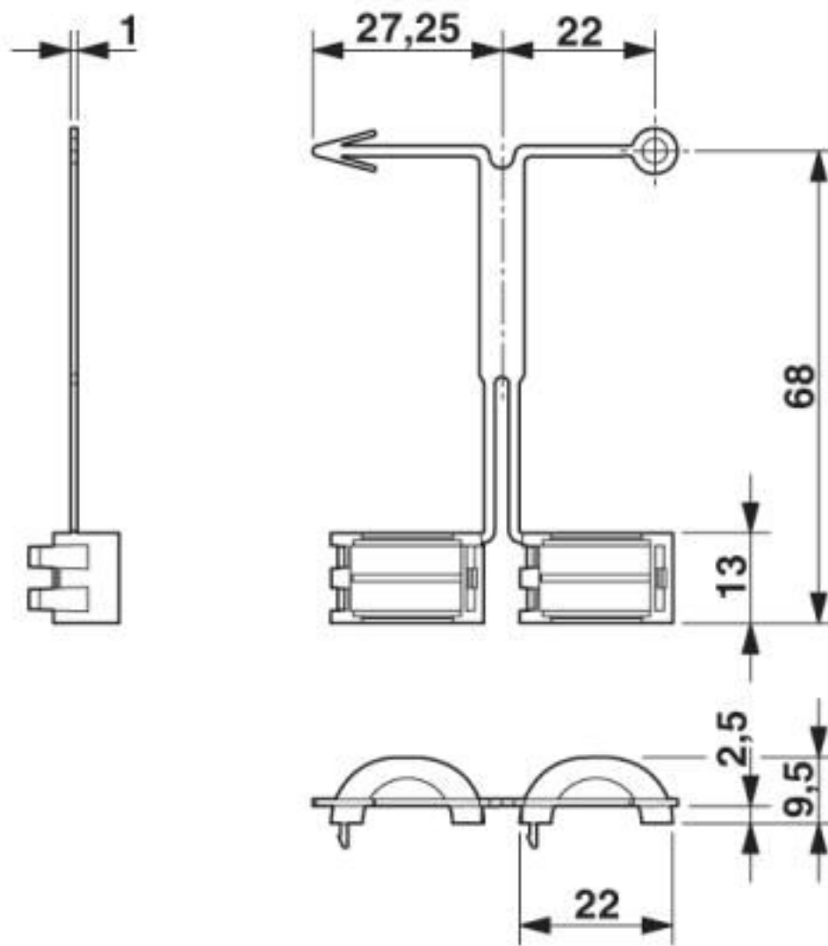
Dimensional drawing
