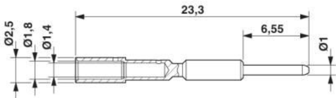
Dimensional drawing
