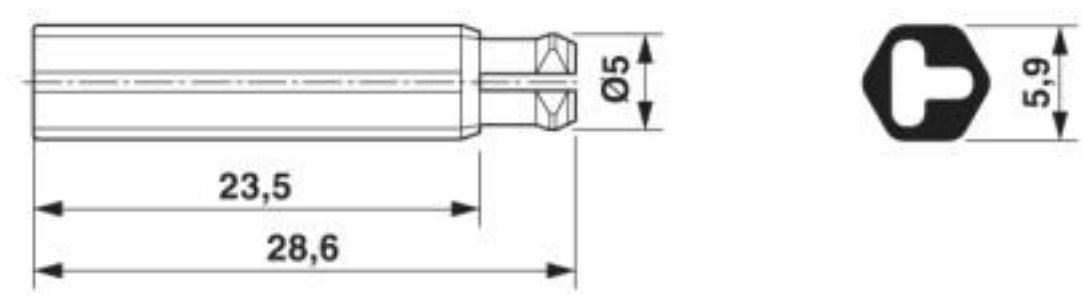
Dimensional drawing
