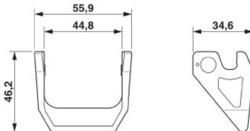
Dimensional drawing
