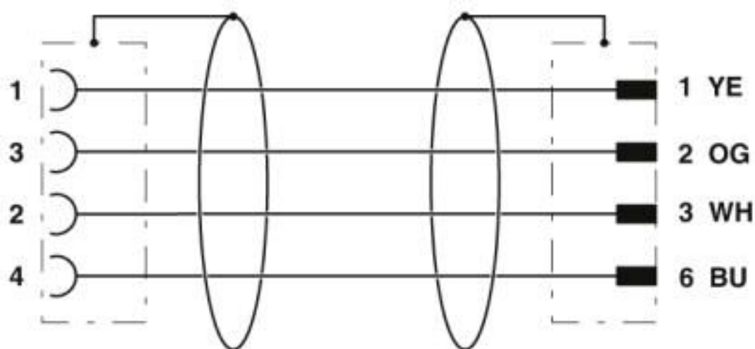
Contact assignment of the M12 socket and the RJ45 plug
