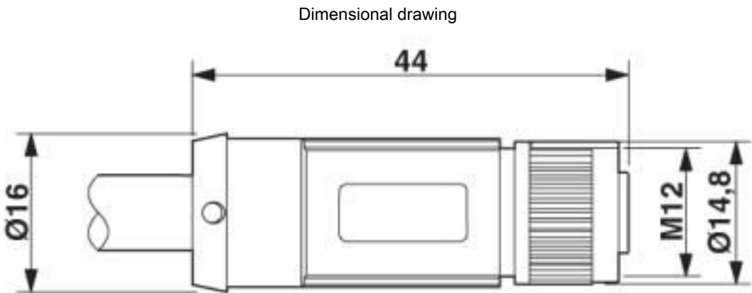
Socket M12-SPEEDCON, straight, shielded
