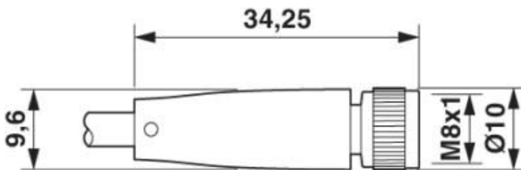
Dimensional drawing
