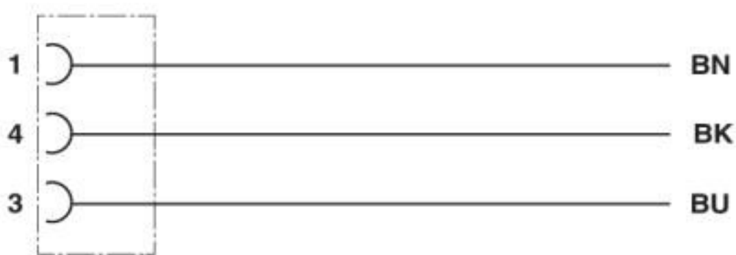
Contact assignment of the M12 socket
