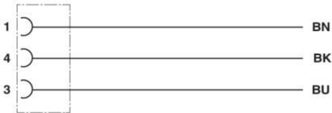
Circuit diagram
