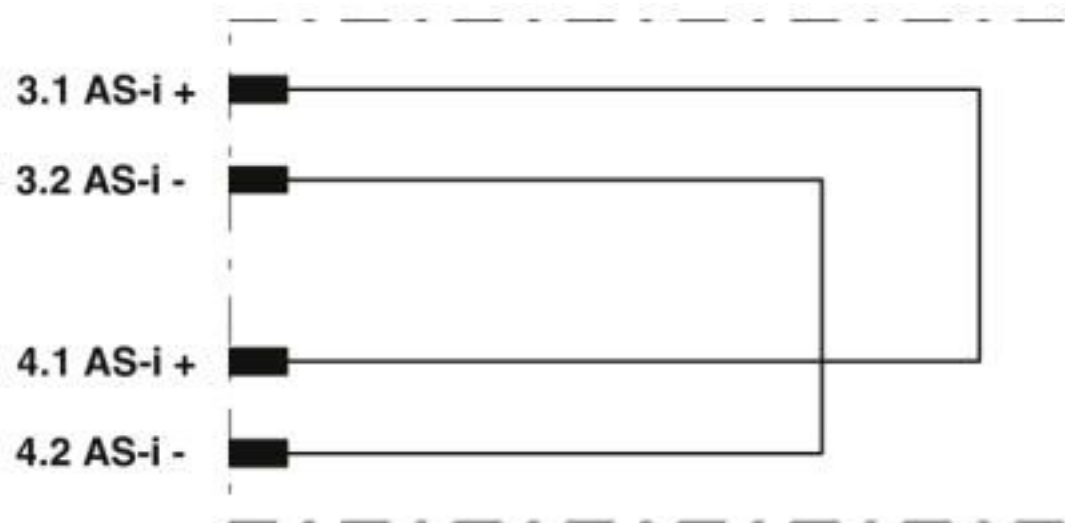
Contact assignment of the AS-Interface distributor
