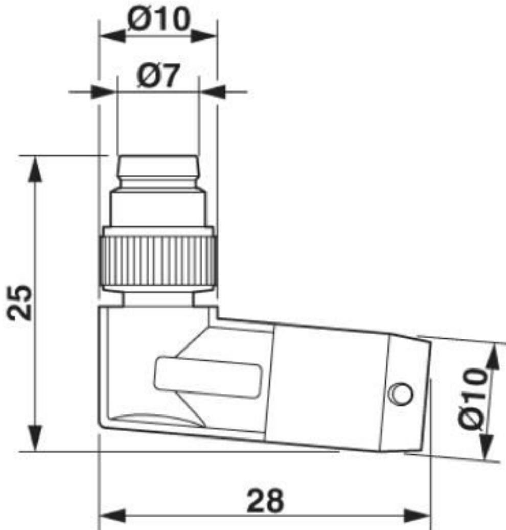
M8 x 1 male plug, angled version
