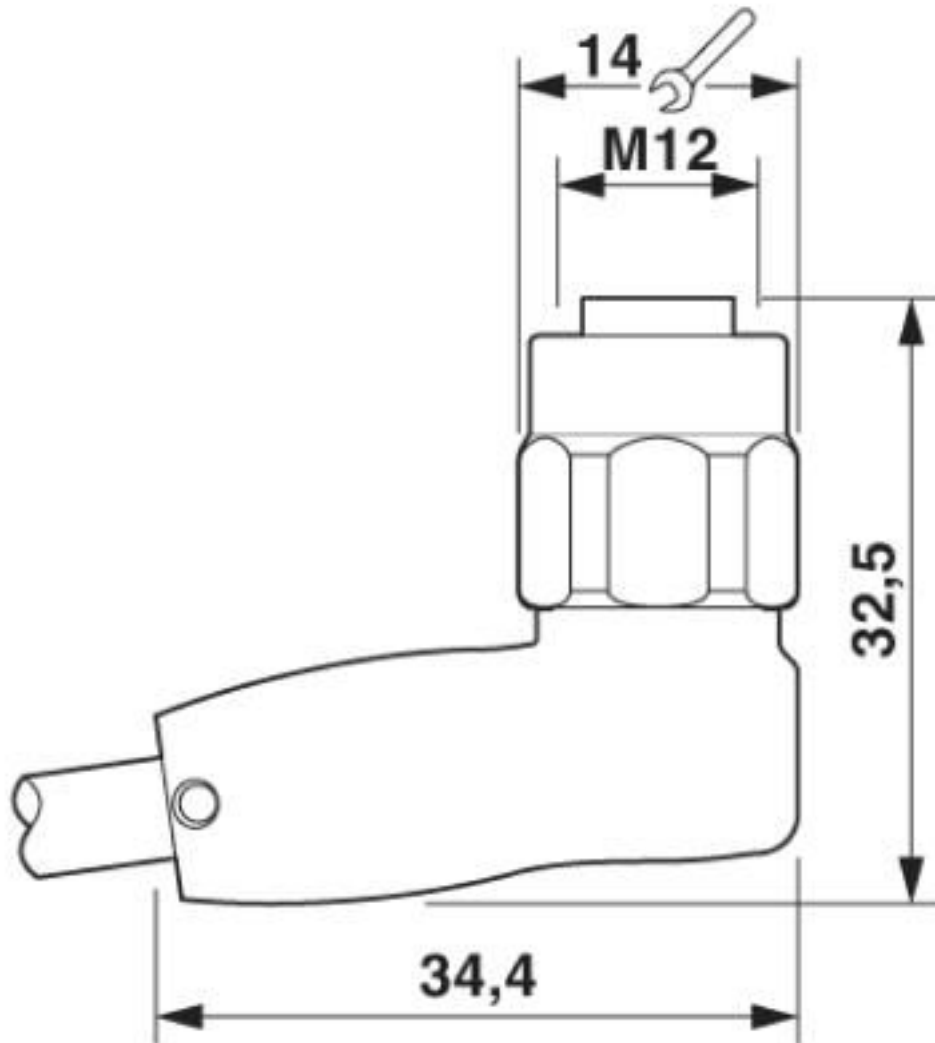
Socket M12 x 1, angled, with LED
